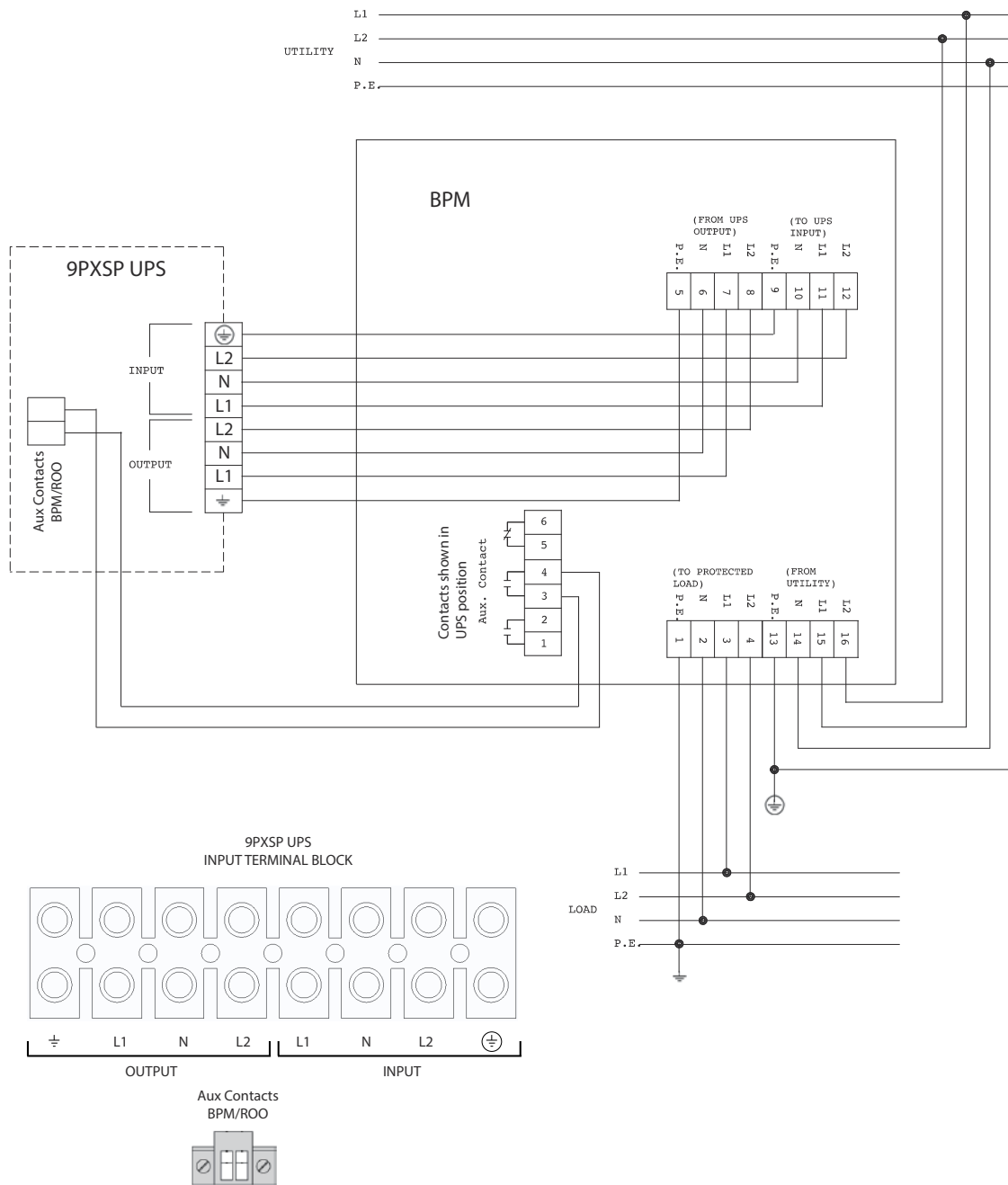
Figure 18. Eaton 9PX SP UPS to BPM Connection Diagram
