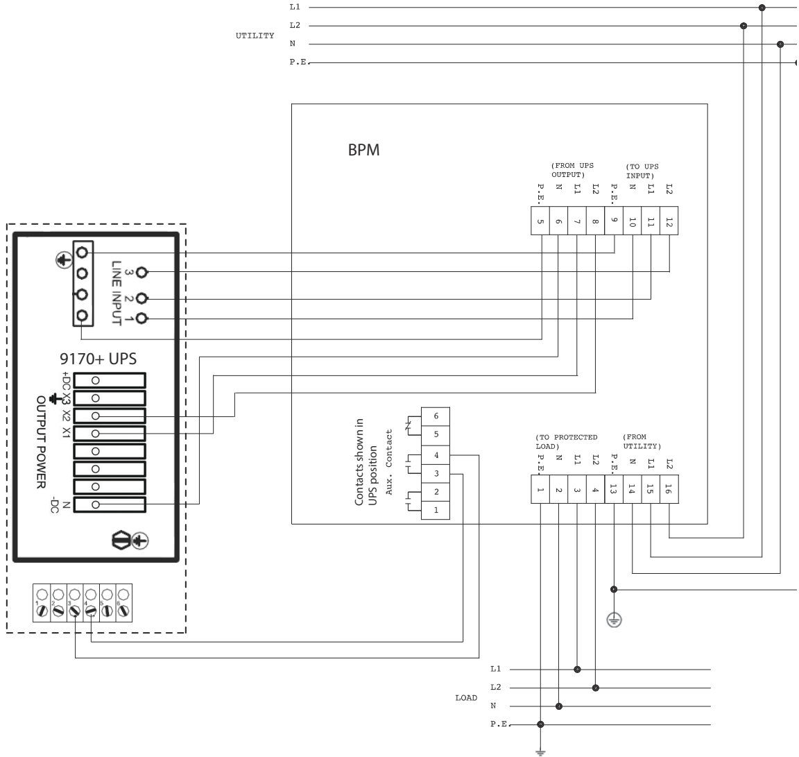
Figure 17. Eaton 9170+ UPS to BPM Connection Diagram
