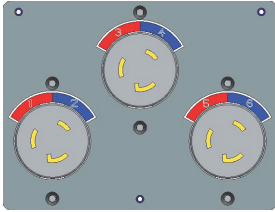
L6-30R
