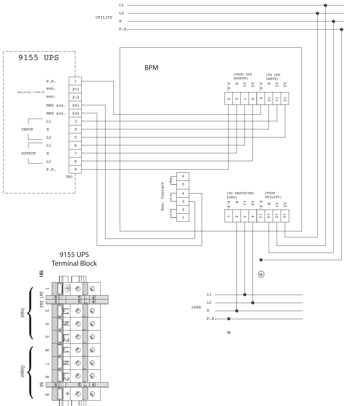
Figure 16. Eaton 9155 UPS to BPM Connection Diagram
